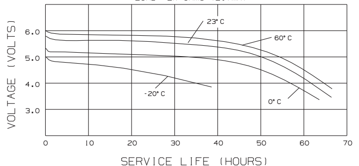
Typical Temperature Characteristics K28L
