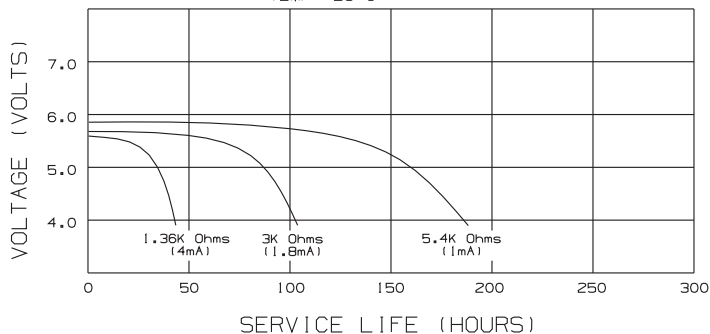
Typical Pulse Discharge Characteristics K28L
